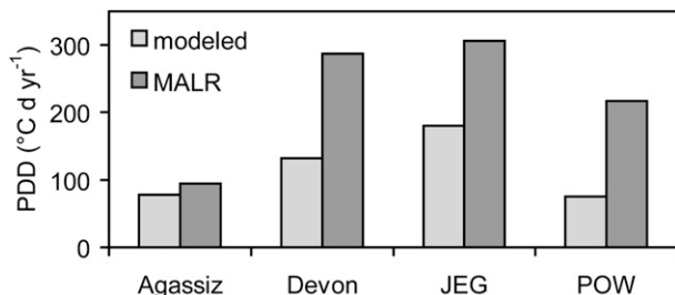
FIG. 11. The 1994–2006 area averaged mean annual PDDs for the Agassiz Ice Cap, Devon Island Ice Caps, JEG, and POW derived from near-surface temperature fields downscaled from NARR 750T using daily modeled and a constant lapse rate set equal to the MALR ( 6.5^{\circ}\text{C km}^{-1} ).
